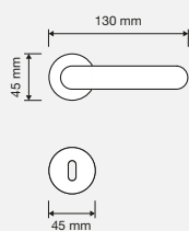
COD. 745 RB 110
