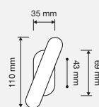
COD. 745 MX
